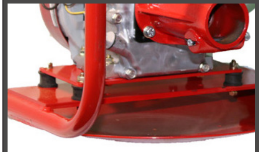
Rubber Mounts
